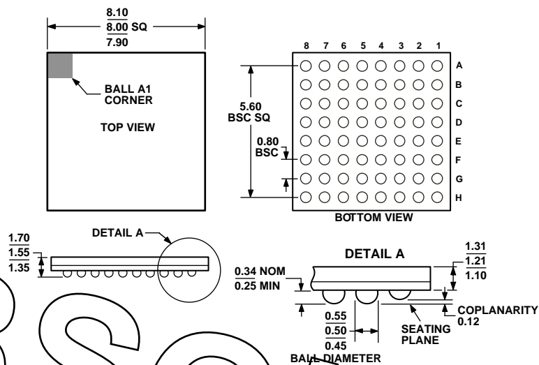
Figure B3. 64-Lead Chip Scale Package Ball Grid Array [CSP_BGA] (BC-64-1) Dimensions shown in millimeters
